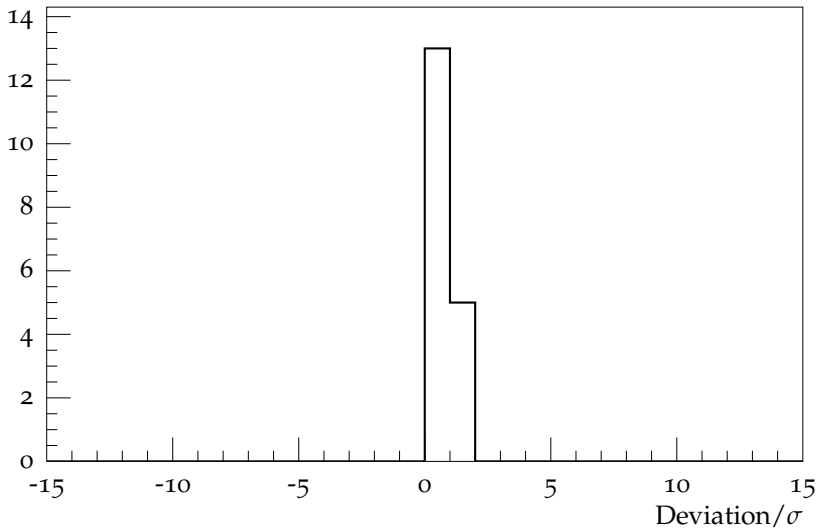
Pull for Transverse \sum p_{\perp} density vs. p_{\perp}^{\text{trk1}} , \sqrt{s} = 7 TeV
