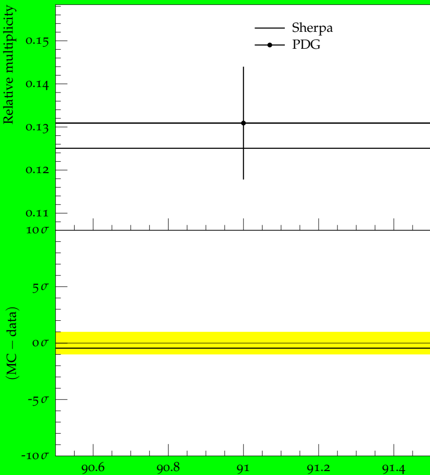
Ratio (w.r.t. \pi^\pm ) of mean K^+ multiplicity
