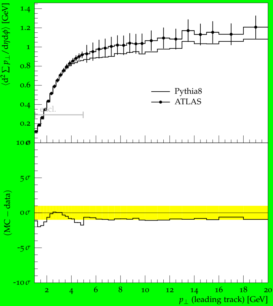
Transverse \Sigma p_{\perp} density vs. p_{\perp}^{\text{trk1}} , \sqrt{s} = 7 TeV
