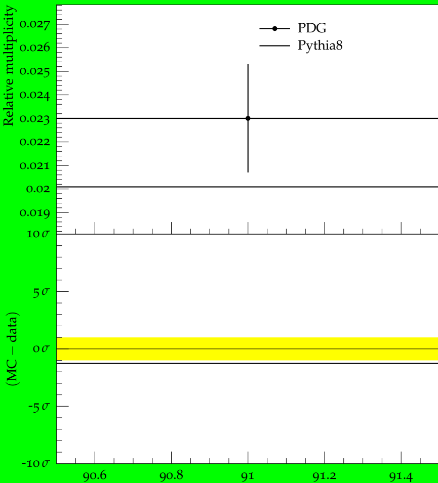
Ratio (w.r.t. \pi^\pm ) of mean \Lambda multiplicity
