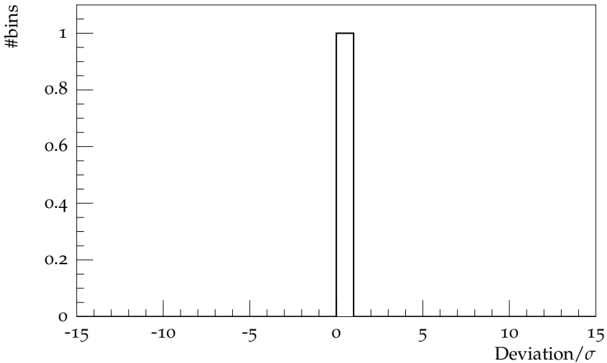
Pull for Mean \pi^+/\pi^- multiplicity
