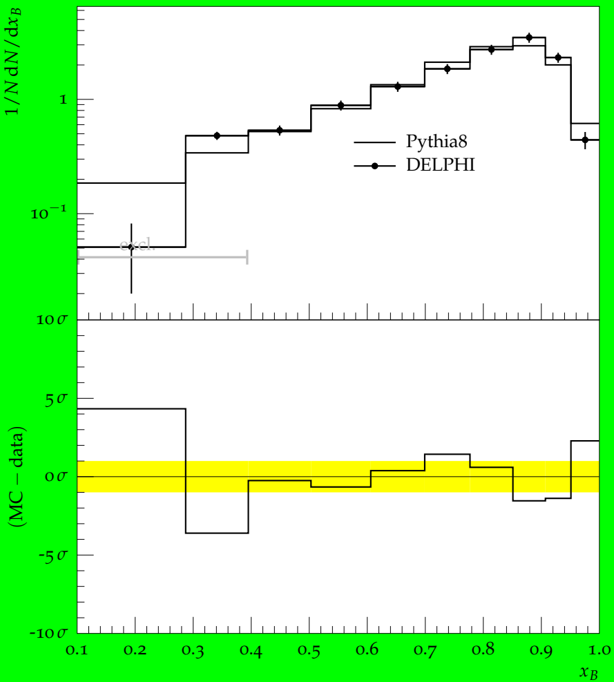
b quark fragmentation function f(x_B^{\text{prim}})
