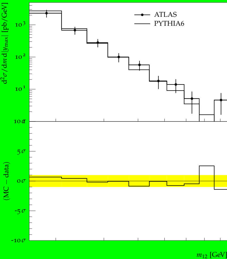
Dijet mass spectrum for 0.3 < |y_{\text{max}}| < 0.8 . anti-KT, R = 0.4 .
