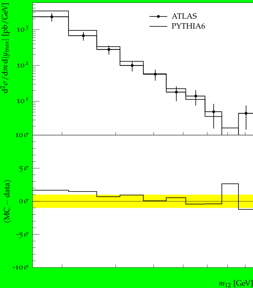
Dijet mass spectrum for 0.3 < |y_{\max}| < 0.8 . anti-KT, R = 0.4 .
