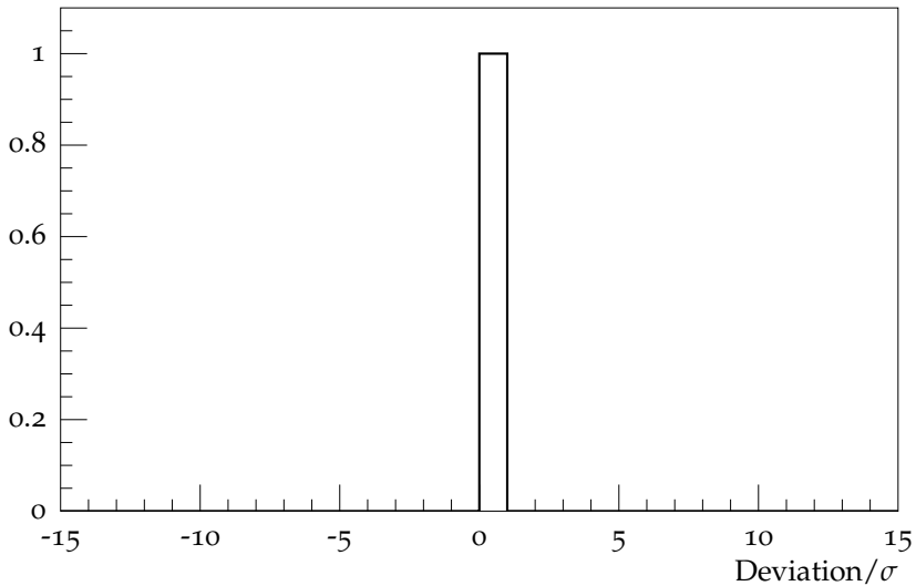
Pull for Ratio (w.r.t. \pi^\pm ) of mean p multiplicity
