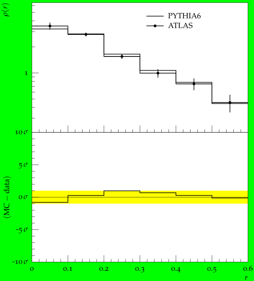
Jet shape \rho for p_{\perp} \in 30\text{--}40\text{ GeV} , y \in 0.0\text{--}2.8
