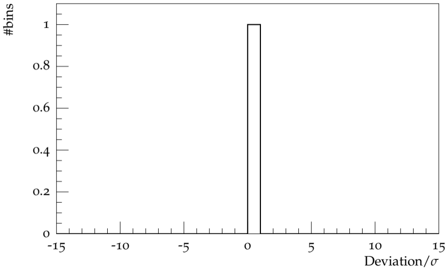
Pull for Ratio (w.r.t. \pi^\pm ) of mean \Lambda multiplicity
