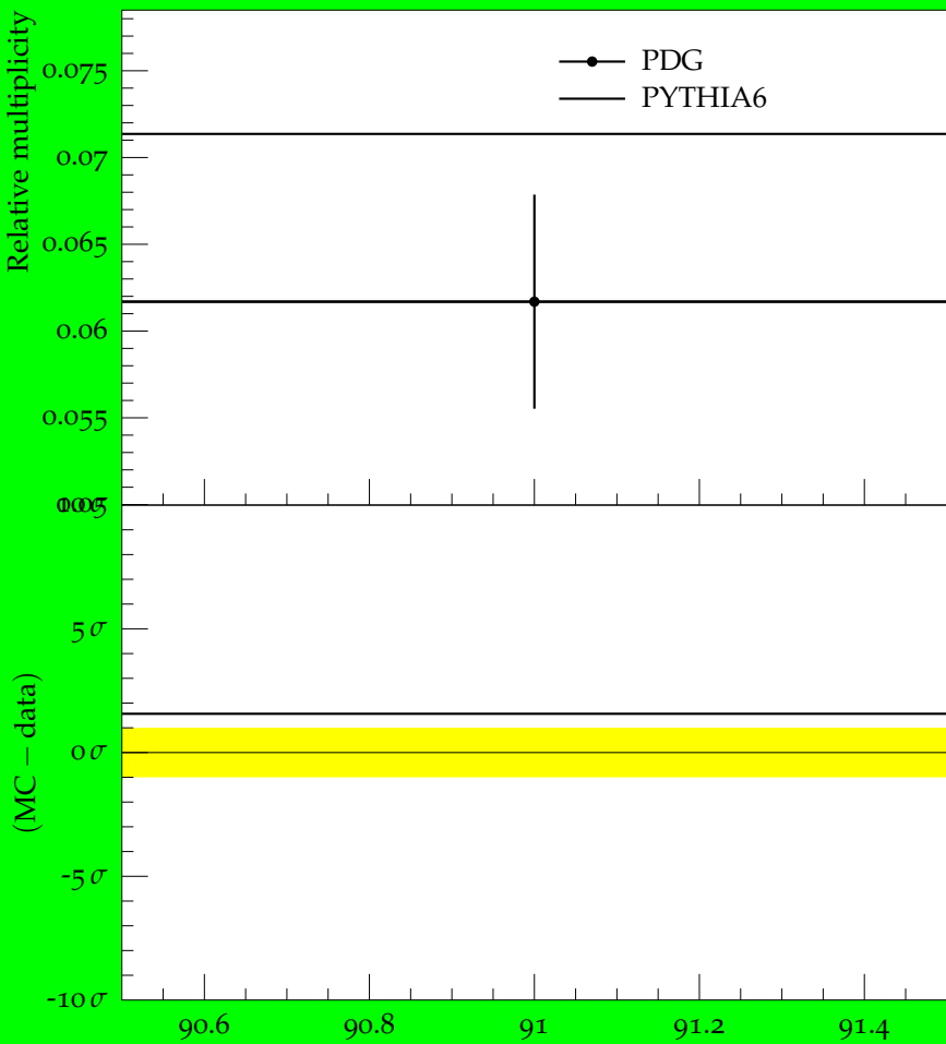
Ratio (w.r.t. \pi^\pm ) of mean p multiplicity
