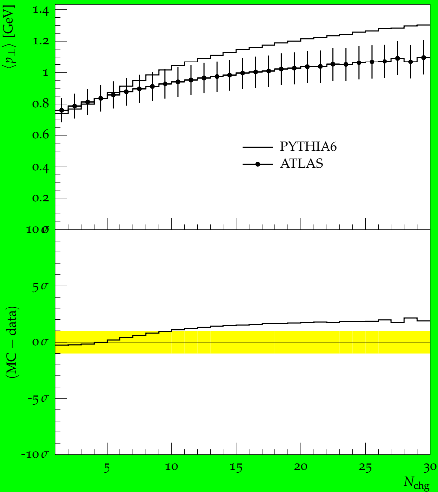
Transverse \langle p_{\perp} \rangle vs. N_{\text{chg}} , \sqrt{s} = 7 TeV
