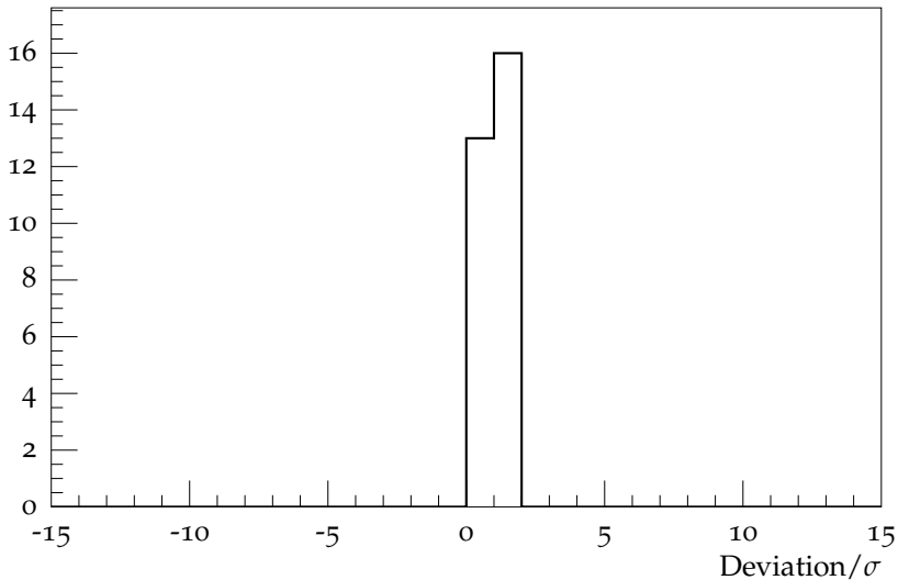
Pull for Transverse \langle p_{\perp} \rangle vs. N_{\text{chg}} , \sqrt{s} = 7 TeV
