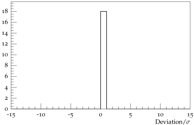
Pull for Transverse N_{\text{chg}} density vs. p_{\perp}^{\text{trk1}} , \sqrt{s} = 7 TeV
