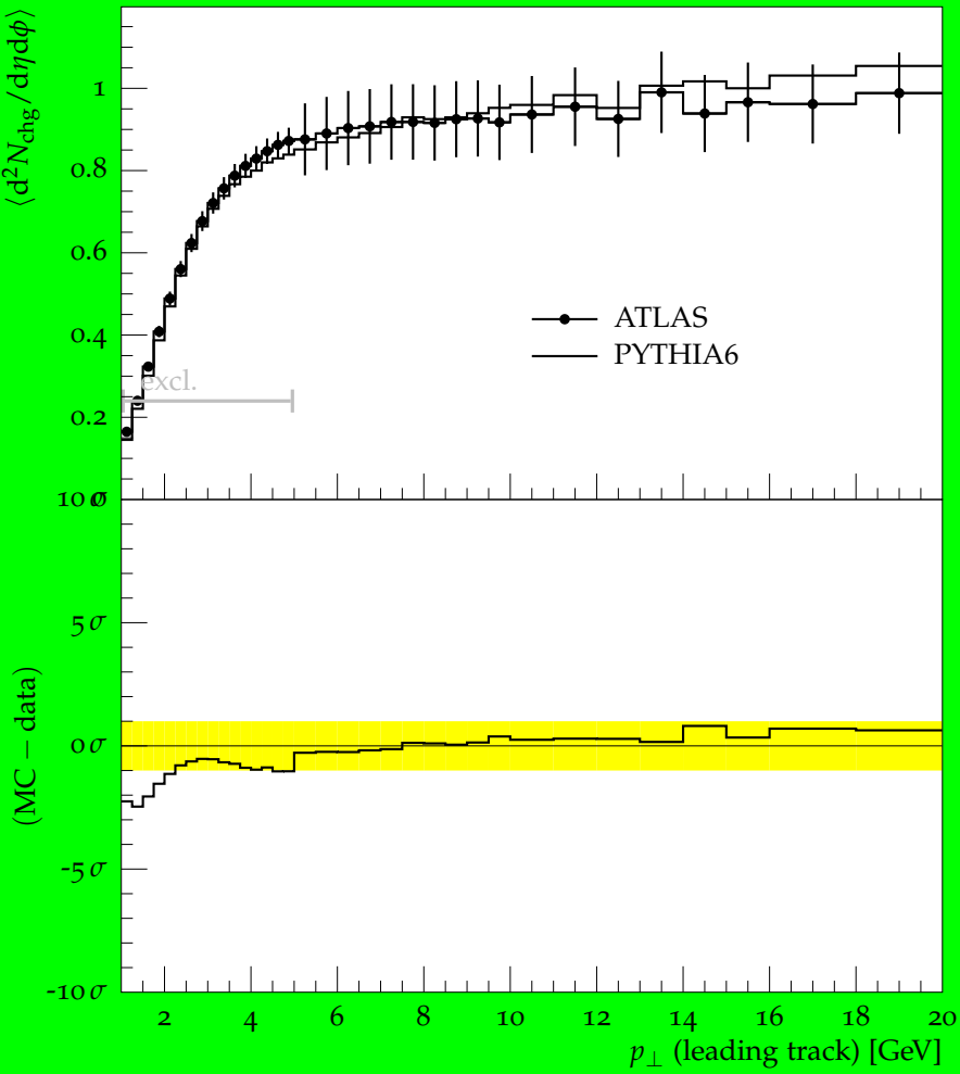
Transverse N_{\text{chg}} density vs. p_{\perp}^{\text{trk1}} , \sqrt{s} = 7 TeV
