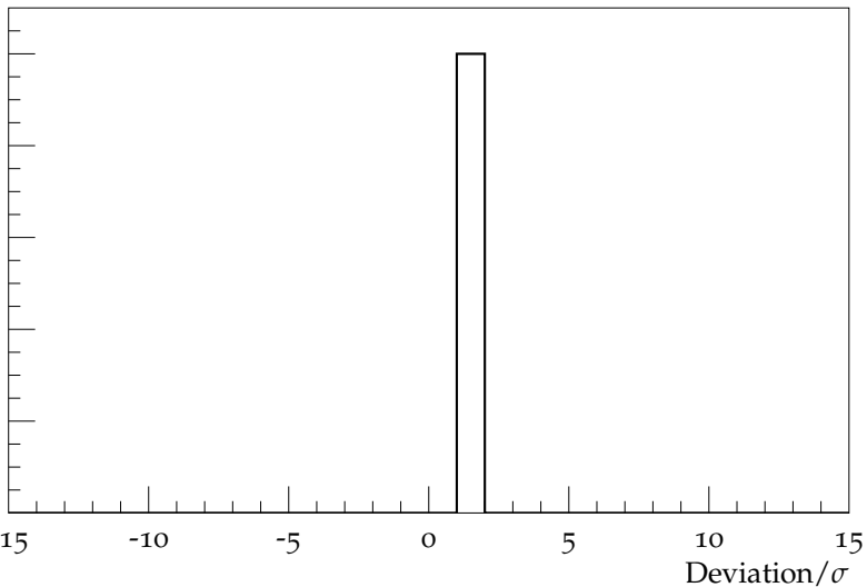
Pull for Mean K^+ / K^- multiplicity
