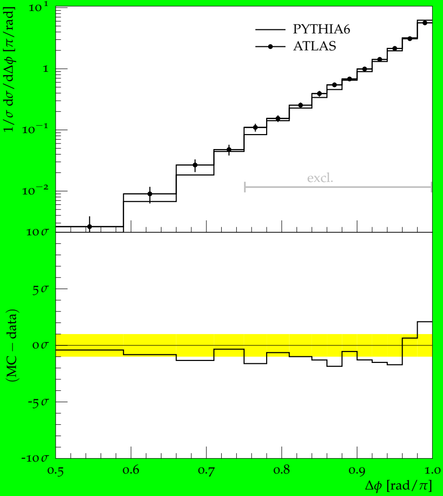
Dijet azimuthal decorrelations for 310 < p_{\perp}^{\text{max}}/\text{GeV} < 400
