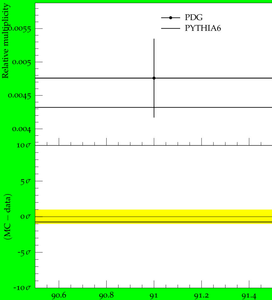
Ratio (w.r.t. \pi^\pm ) of mean \Sigma^- multiplicity
