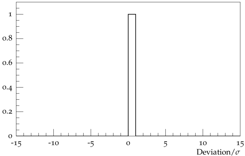
Pull for Ratio (w.r.t. \pi^\pm ) of mean \Sigma^0 multiplicity
