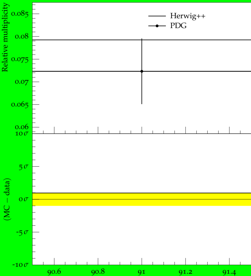
Ratio (w.r.t. \pi^\pm ) of mean \rho^0(770) multiplicity
