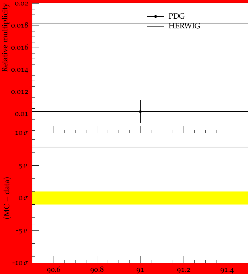
Ratio (w.r.t. \pi^\pm ) of mean \Sigma^\pm multiplicity
