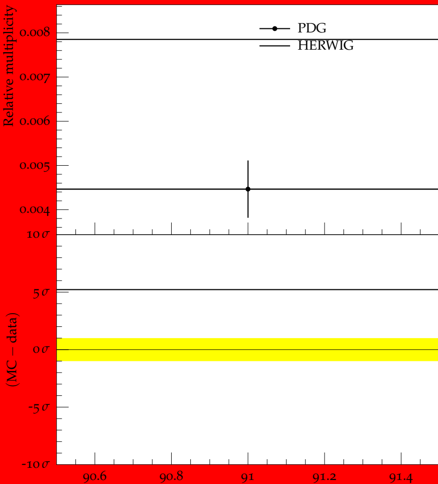
Ratio (w.r.t. \pi^\pm ) of mean \Sigma^0 multiplicity
