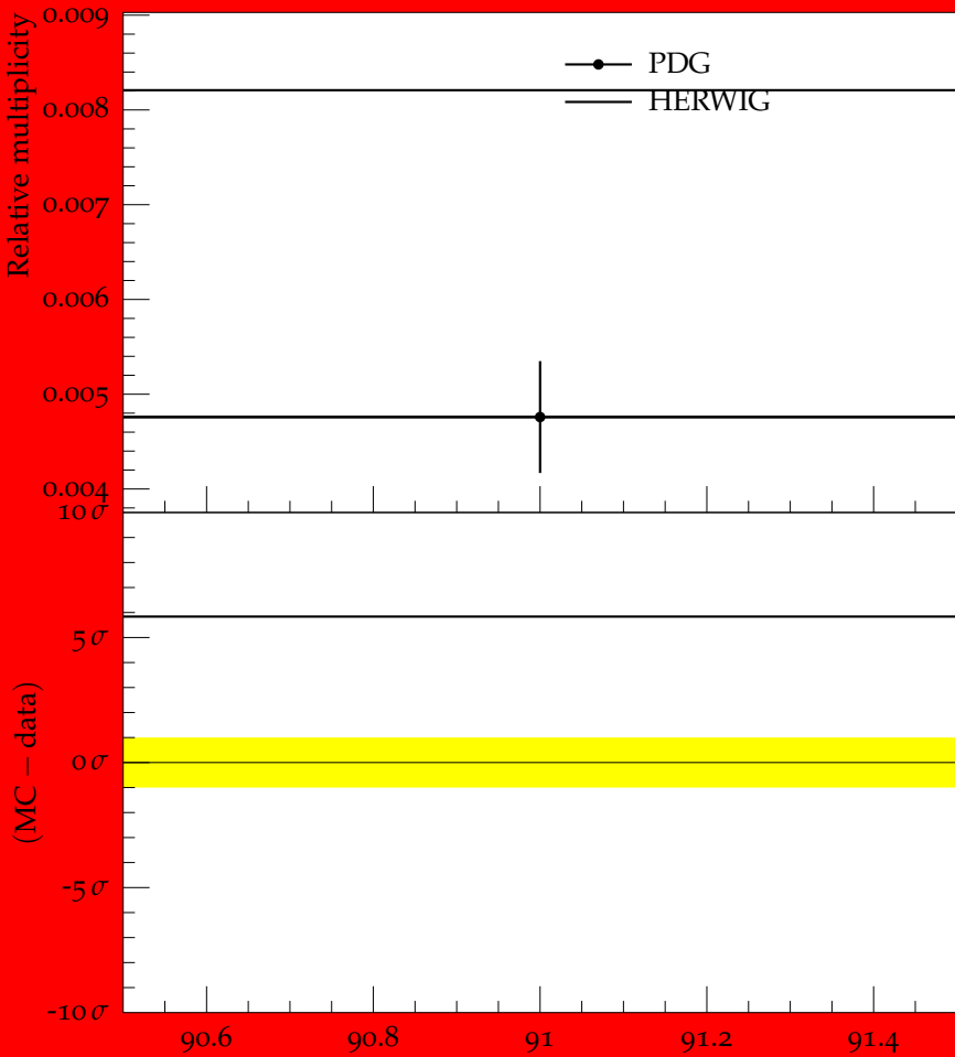
Ratio (w.r.t. \pi^\pm ) of mean \Sigma^- multiplicity
