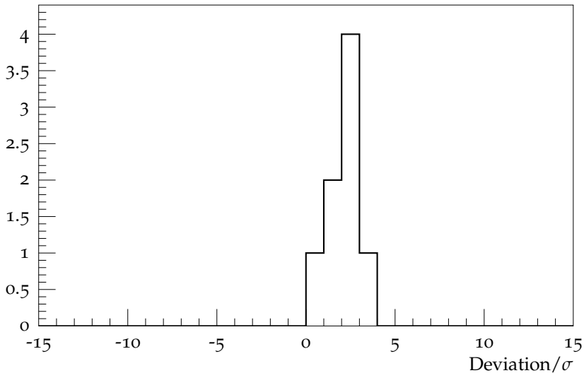
Pull for b quark fragmentation function f(x_B^{\text{prim}})
