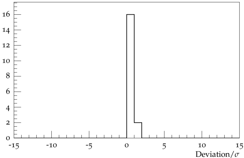
Pull for Muon channel ( |y_Z| < 1 )
