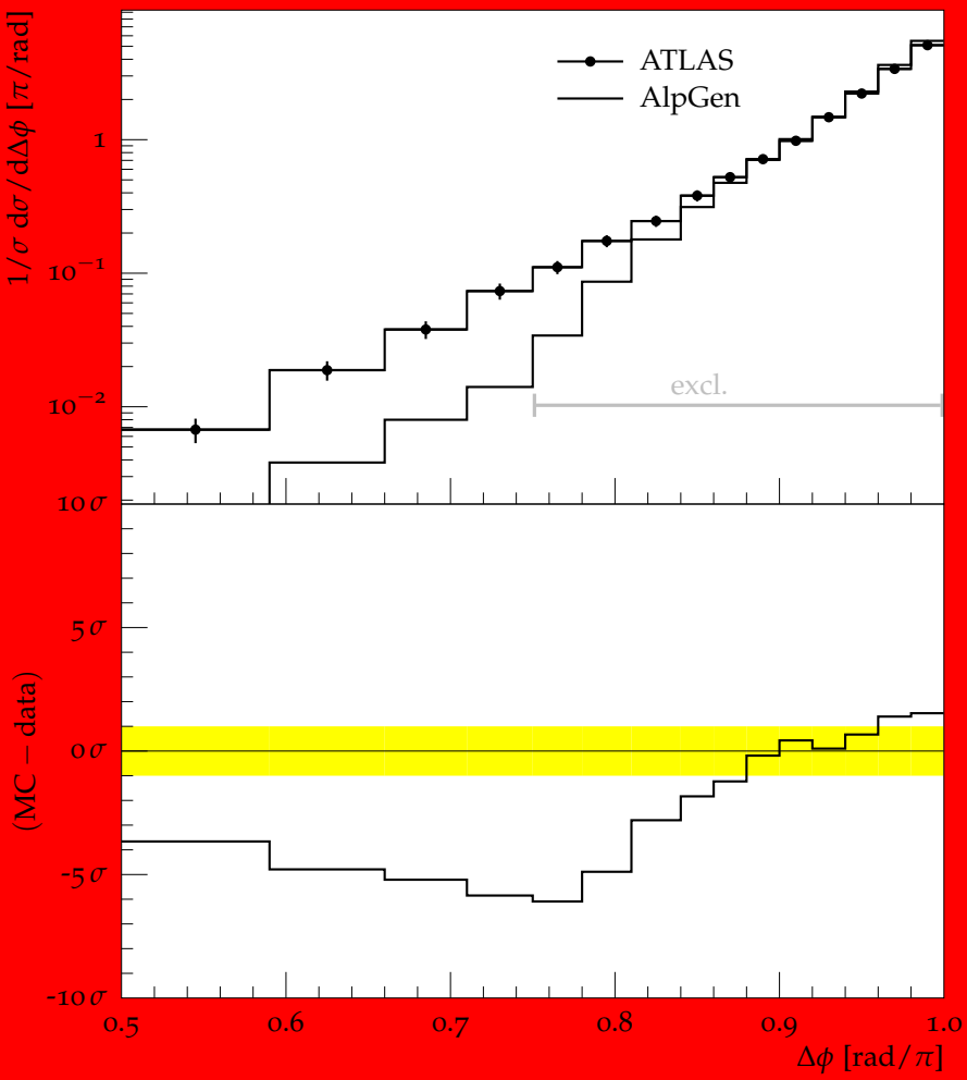
Dijet azimuthal decorrelations for 110 < p_{\perp}^{\text{max}}/\text{GeV} < 160
