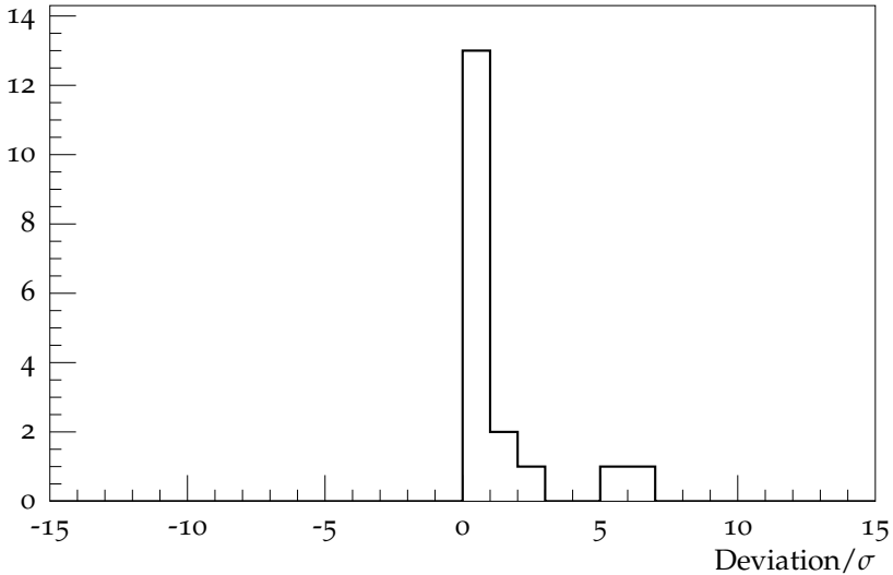
Pull for Muon channel ( 1 < |y_Z| < 2 )
